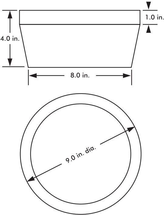
Figure B8. Large head probe
